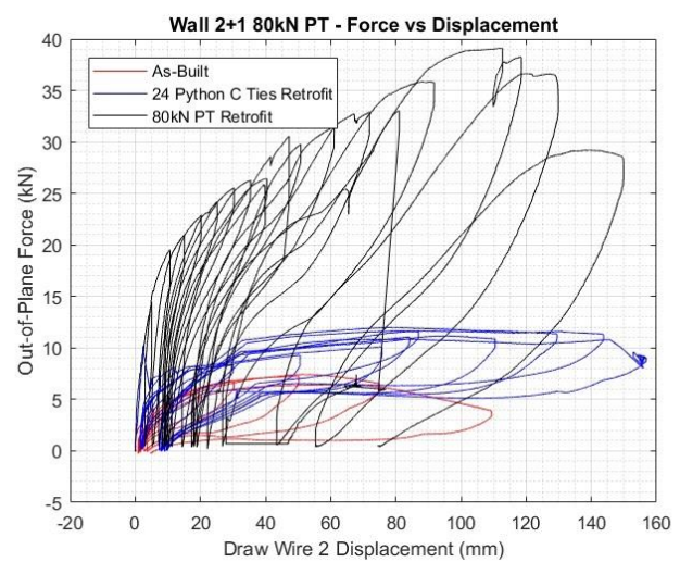
(b) 80 kN PT: out-of-plane force vs displacement
