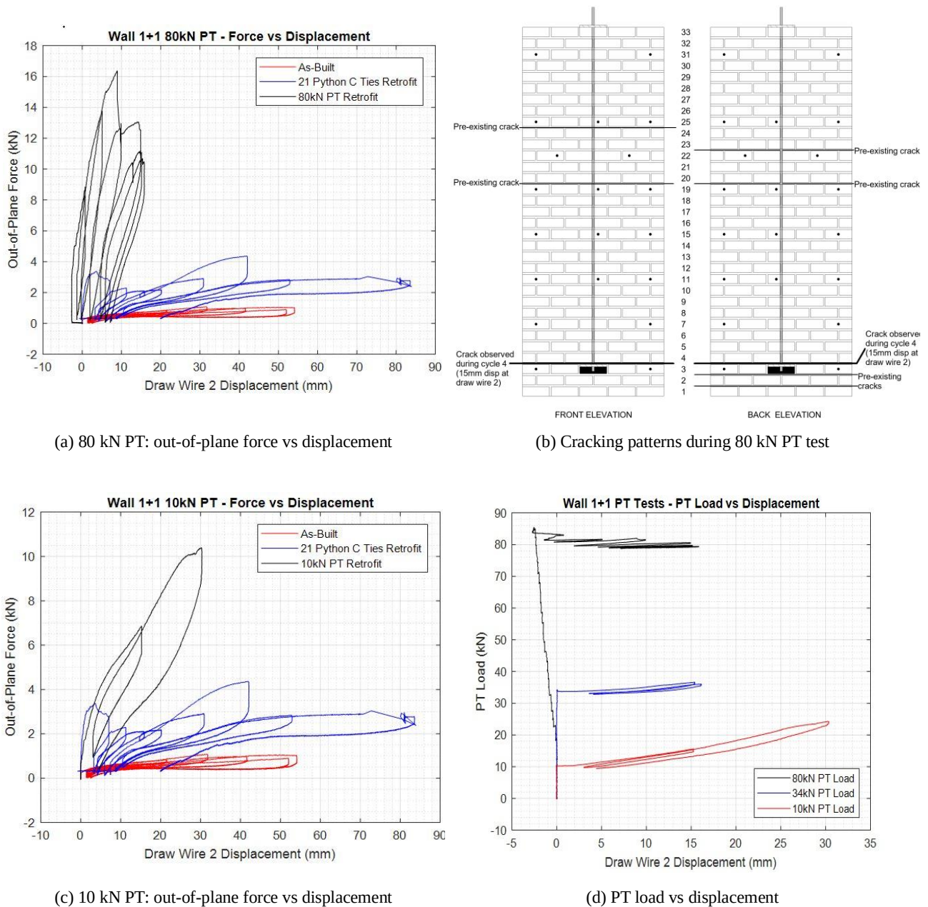
Figure 6: Wall 1+1 Semi-Cyclic Testing
