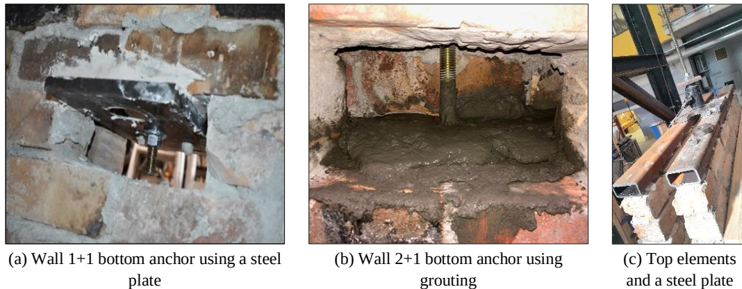
Figure 2: Post-tensioned anchor connections
