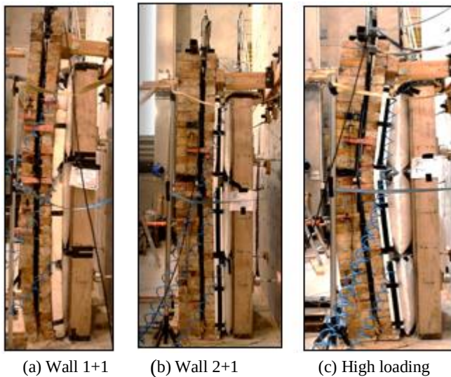
Figure 5: Loading of test walls
